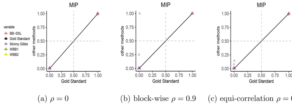
Figure 5. Posterior means of \gamma_i 's (i.e., a marginal inclusion probabilities) in high-dimensional settings with n = 100, p = 1000 . We set \lambda_0 = 50, \lambda_1 = 0.05 .
