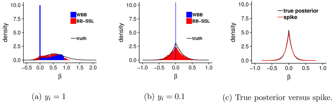
Figure 1. True and WBB approximated posterior distribution \pi(\beta_i | y_i) under the separable SSL prior with \lambda_0 = 5 , \lambda_1 = 0.1 and \theta = 0.2 and a Gaussian sequence model y_i = x_i + \epsilon_i/\sqrt{n} with n = 10 . Red bins represent BB-SSL pseudo-posterior, blue bins represent WBB pseudo-posterior (with a random prior weight), black line is the true posterior and \alpha = 2.5 . The plot (c) is for the same setting except with \lambda_0 = 10 .
