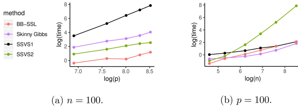
Figure 2. Average running times (in seconds on a log scale) for 100 iterations of each algorithm based 10 independent runs. Covariates are all correlated with a correlation coefficient \rho = 0.6 . Signals are (2, 3, -3, 4) and we set \lambda_0 = 200, \lambda_1 = 0.05, a = 1, b = p . BB-SSL is initialized at the SS-LASSO solution obtained with a sequence of \lambda_0 's (an equi-spaced series of length 50 starting at \lambda_1 = 0.05 and ending at \lambda_0 = 200 ).
