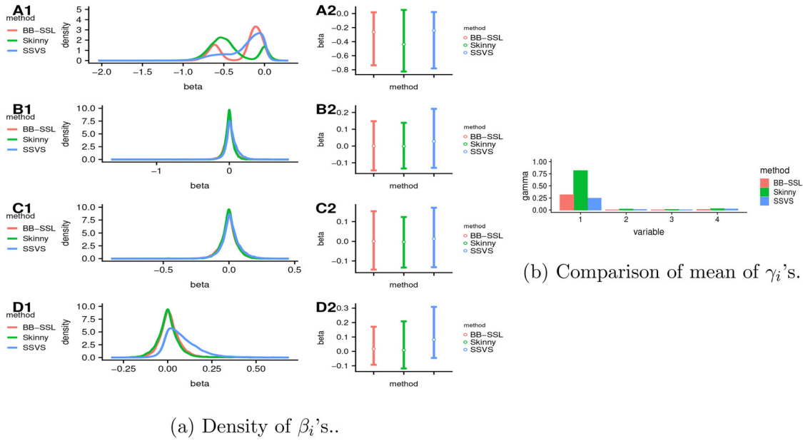
Figure 8. Plots for Life Cycle Savings Data. We choose \lambda_0 = 20, \lambda_1 = 0.05 . SSVS is initialized at the LASSO solution (with the regularization parameter chosen by cross-validation). The weight distribution for BB-SSL uses \alpha = 2 \log \frac{(1-\theta)\lambda_0}{\theta\lambda_1} = 14 .
