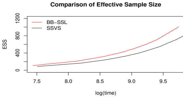
Figure 9. Effective sample size comparison for ISMS Durable Goods Dataset 2. We choose \lambda_0 = 100, \lambda_1 = 0.05 . Red line is BB-SSL with \alpha = 2 \log \frac{(1-\theta)\lambda_0}{\theta\lambda_1} \approx 15 and black line is SSVS initialized at origin.
