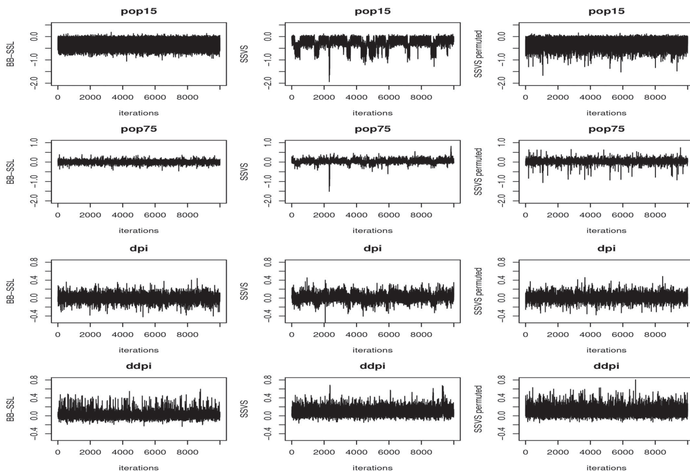
Figure 7. Trace plots for the Life Cycle Savings data. We choose \lambda_0 = 20, \lambda_1 = 0.05 . The first column is the BB-SSL traceplot with weight distribution \alpha = 2 \log \frac{(1-\theta)\lambda_0}{\theta\lambda_1} = 14 , the second column is thinned SSVS traceplot chain with a LASSO initialization (regularization parameter chosen by cross-validation). The third column is the same SSVS chain only with samples permuted.
