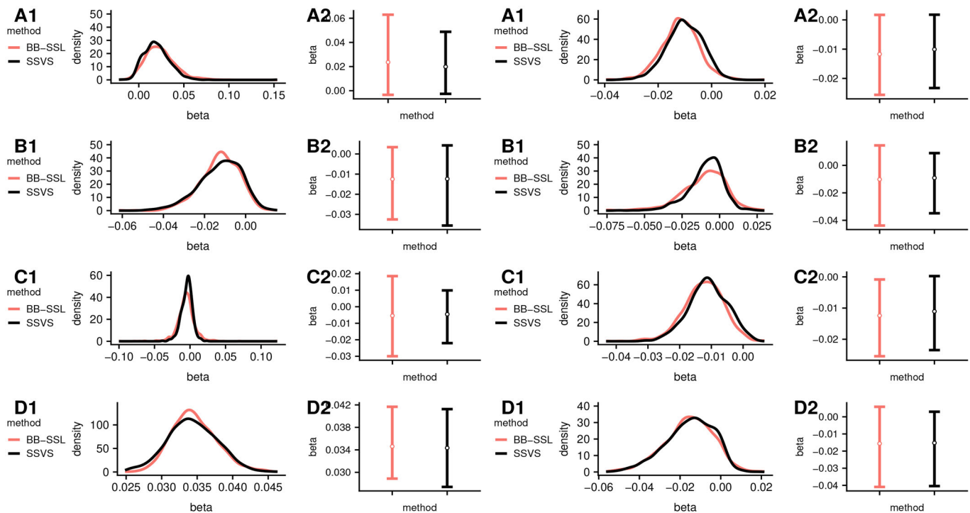
Figure 10. Posterior density and credible intervals for the selected \beta_j 's. From left to right, top to bottom they correspond to "S-SAL-TOT60M", "S-U-CLS-NBR-12MO", "PH-HOLIDAY-MAILER-RESP-SA", "PROMO-NOV-SALES", "S-SAL-FALL-24MO", "S-TOT-CAT \times treatment", "C-ESP-RECT \times treatment", "S-CNT-TOT24M \times treatment". We set \lambda_0 = 100 , \lambda_1 = 0.05 , a = 1 , b = 273 . We set \alpha = 2 \log \frac{(1-\theta)\lambda_0}{\theta\lambda_1} \approx 15 .
